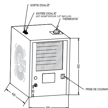
Installation plans
