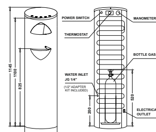
Installation drawing
