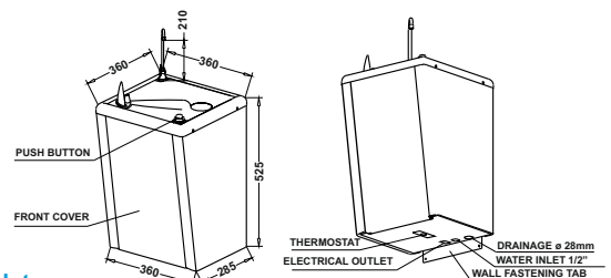
Installation drawing
