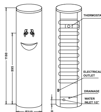
Installation drawing
