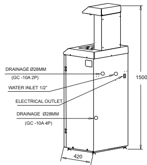
Installation drawings
