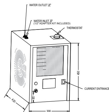
Installation drawings
